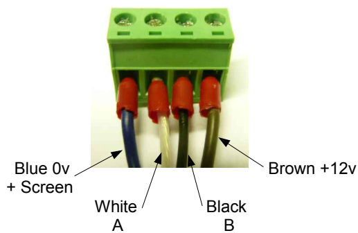
Terminal Plug Wiring
