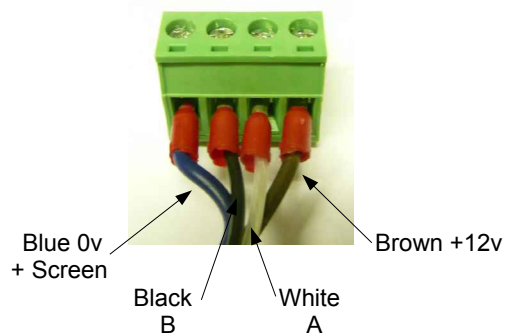
Relay Plug Wiring
